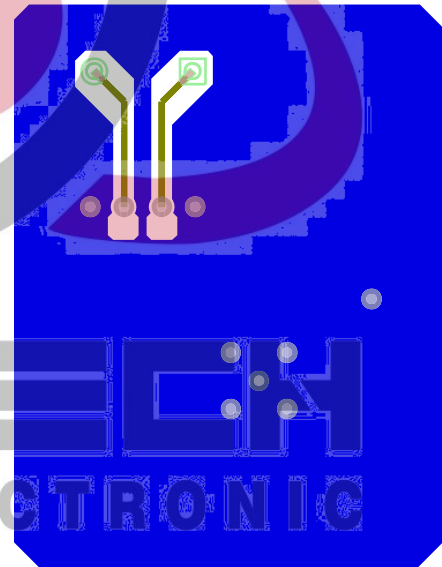
Figure 116. ADE7880 Bottom Layer Printed Circuit Board
