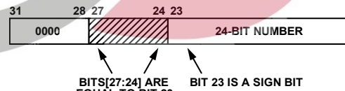
Figure 44. 24-Bit xIGAIN Transmitted as 32-Bit Words
