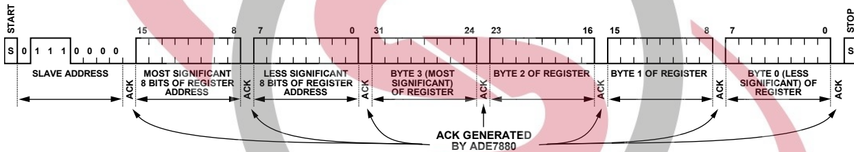
Figure 103. I 2 C Write Operation of a 32-Bit Register
