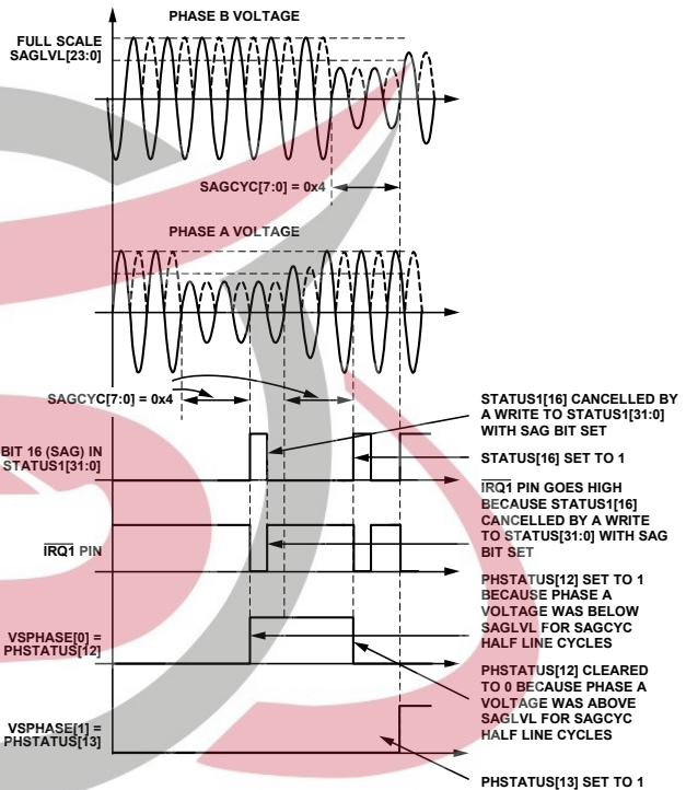
Figure 58. SAG Detection
