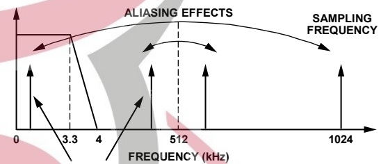
Figure 41. Aliasing Effects
