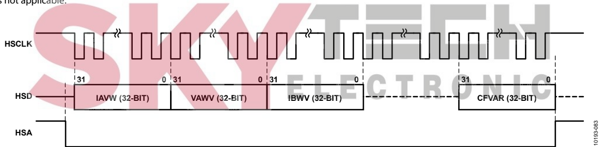
Figure 111. HSDC Communication for HGAP = 0, HXFER[1:0] = 00, and HSAPOL = 0; HSIZE Is Irrelevant
