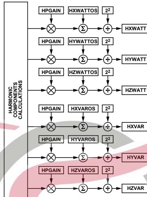
Figure 89. Harmonic Active and Reactive Powers Signal Processing
